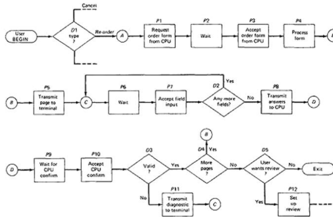
Figure 3.1: An Example of a Transaction Flow
