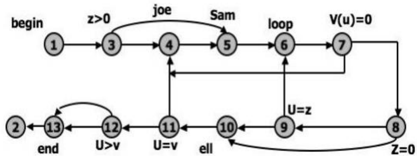
Figure 1.5: Simplified Flowgraph Notation
