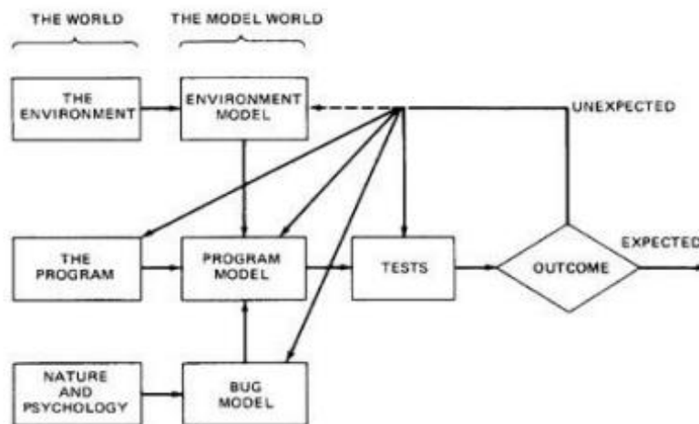
Figure 1.1: A Model for Testing
