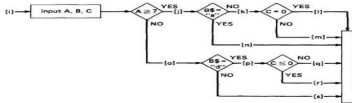
Figure 1.12: Single Link Marker Instrumentation
