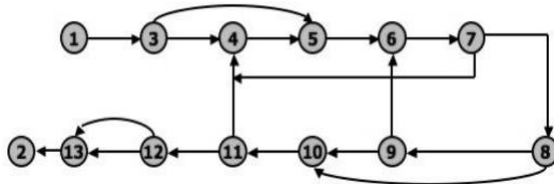
Figure 1.6: Even Simplified Flowgraph Notation
