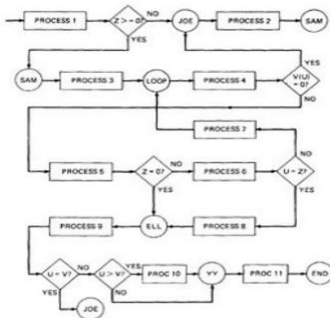
Figure 1.4: Control Flowgraph for example in Figure 1.2
