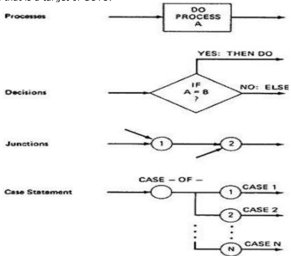
Figure 1.1: Flowgraph Elements
