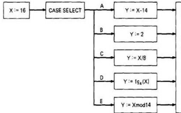
Figure 1.II: Coincidental Correctness
