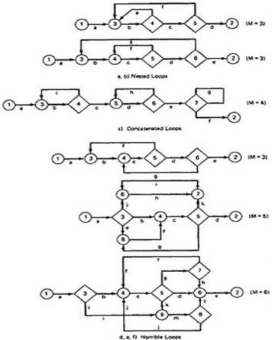
Figure 2.10: Example of Loop types
