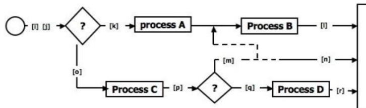
Figure 2.14: Double Link Marker Instrumentation.
