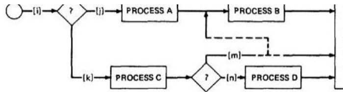
Figure 2.13: Why Single Link Markers aren't enough.
